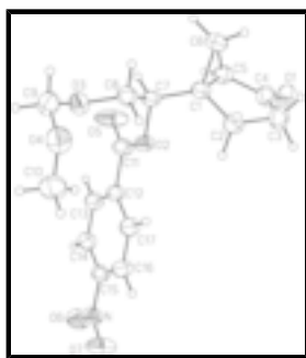
Fig. 2. Perspective view of (V), showing the atom labelling scheme. Non-hydrogen atoms are represented by ellipsoids at the 50% probability level. Hydrogen atoms are shown with arbitrarily small radii.
